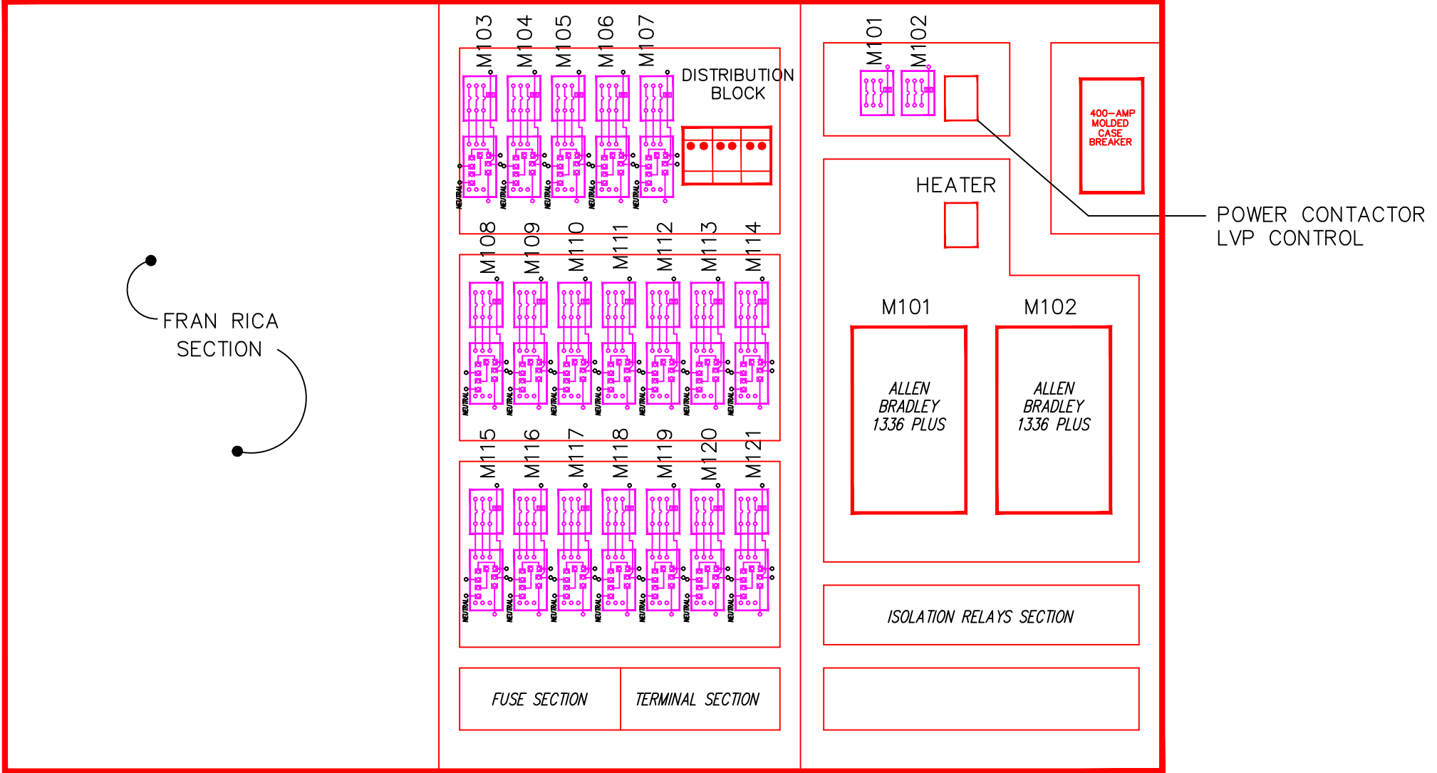
MCC-1 MOTOR CONTROL ELEVATION ARCH D-SIZE SHEET SCALE: NOT TO SCALE (SCALED TO FIT)
